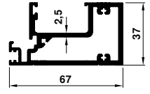
12654 1.623 kg/m
