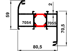
70-7037-7001 1.786 kg/m
