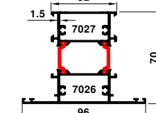
70-7027-7026 1.989 kg/m
