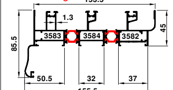
3585-3586 1.289 kg/m
