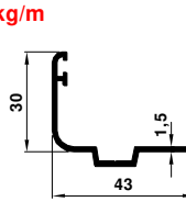
1681 0.340 kg/m
