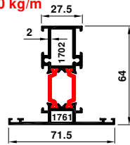
64-6500-6501 1.714 kg/m
