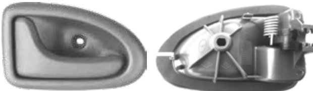
Megane-1 Kapı İç Açma Kolu Sol (Gri) Megane-1 Door Interior Opening Handle Left (Grey)
