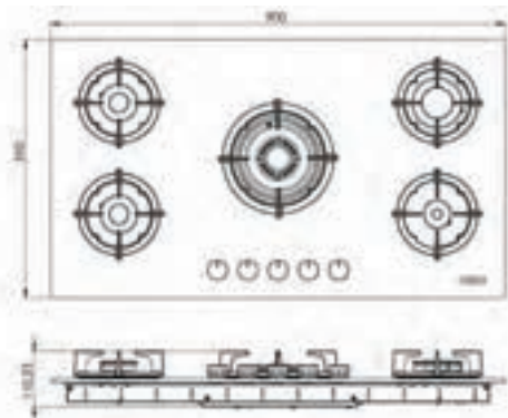
C7-Product Dimensions
